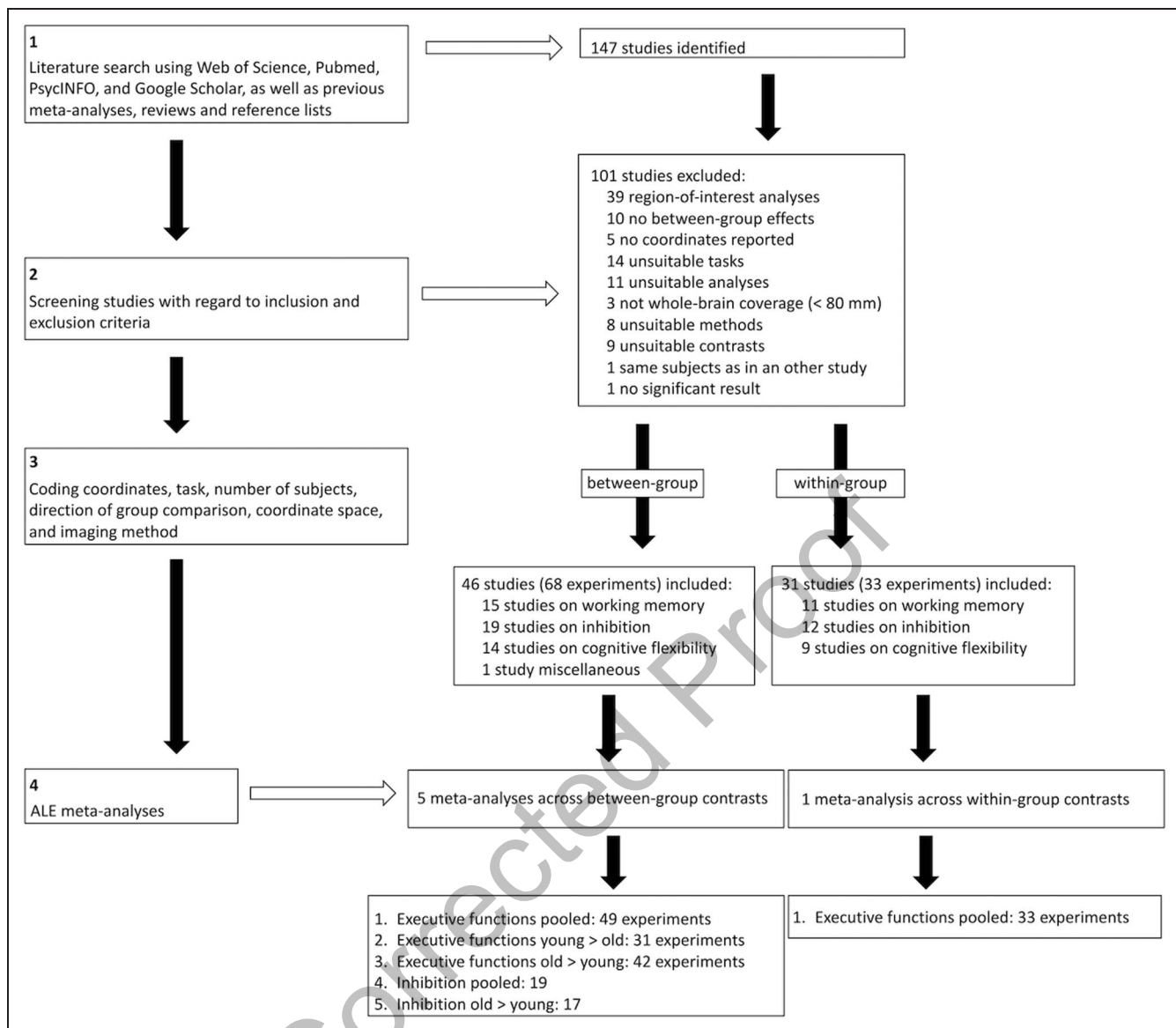
Figure 1. Flowchart of the meta-analysis steps conducted.
